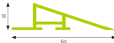
Inner height 18 mm (for mat height 17 mm )
